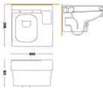
VASO SOSPESO HI TECH WALL HUNG WC HI TECH SONE.20.W01H
