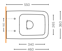
VASO FILO MURO BACK TO WALL WC SCLB.20.F01
