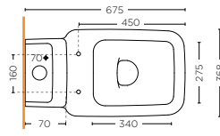
VASO MONOBLOCCO CLOSE COUPLED WC SCLB.20.C01
