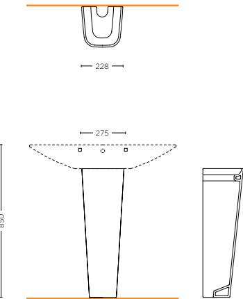
COLONNA PEDESTAL SCLB.PD.10.01
